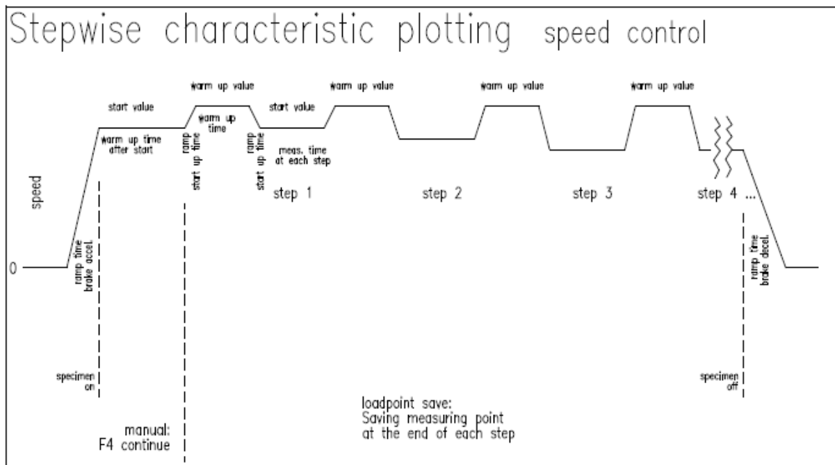
Step characteristic plotting - speed - controlled
